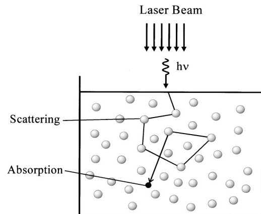
FIG. 3. Physical mechanisms in microstereolithography of concentrated ceramic suspensions: Optical scattering, absorption, and photopolymerization.
