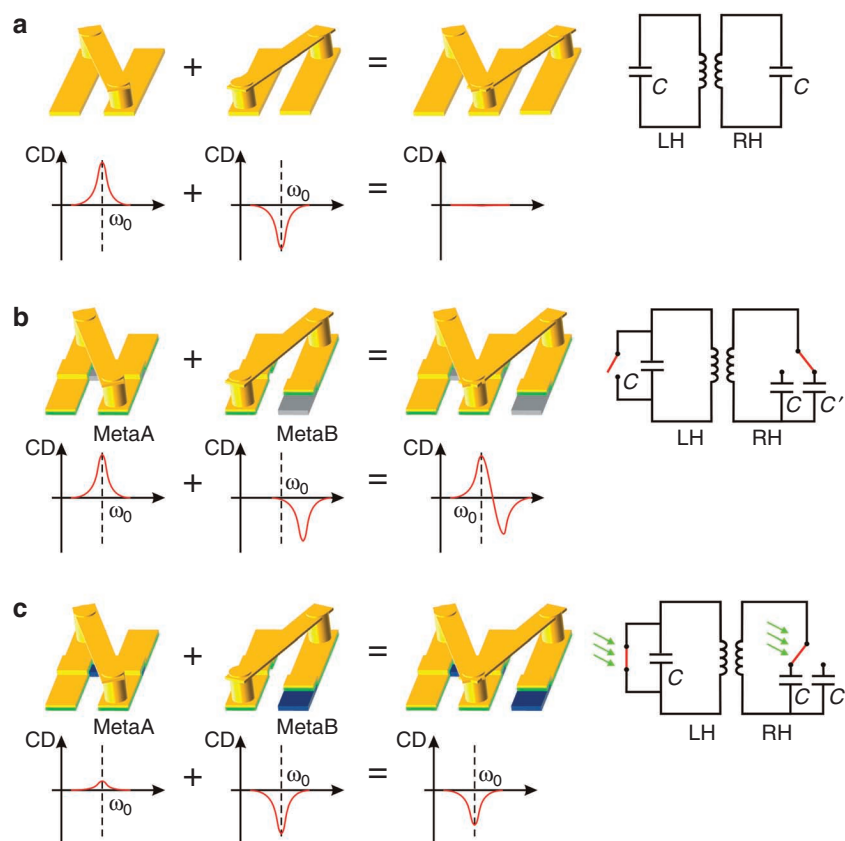
Figure 4 | Schematic design of chiral switching metamaterials illustrating the underlying mechanism. (a) A metamolecule consisting of two meta-atoms of opposite chirality. Each meta-atom is a three-dimensional gold split-ring resonator with its loop tilted relative to the gap, leading to the coupling between the electric and magnetic responses, and consequently, a strong chirality and large CD at its resonance frequency. When combined into a metamolecule, the optical activity arising from the two meta-atoms cancels each other out, resulting in a vanishing circular dichroism spectrum. The metamolecule can be represented by an equivalent circuit consisting of two LC resonators. (b) Silicon pads (gray) are incorporated to the metamolecule. The mirror symmetry is broken, and the metamolecule exhibits chirality at resonance frequencies. The silicon pads also function as the optoelectronic switches in the equivalent circuit. (c) With photoexcitation, photocarriers are generated in the silicon pads, leading to a switching of chirality in the form of reversed circular dichroism.
