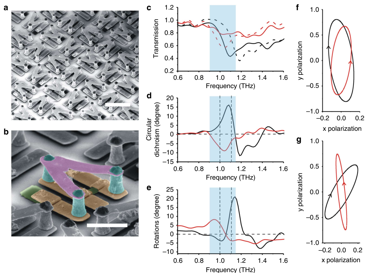
Figure 2 | Experimental demonstration of chiral switching metamaterials. (a,b) Scanning electron microscopy images of the fabricated metamaterial. The period of the metamaterial is 50\ \mu\text{m} , which is far less than the wavelength of the terahertz waves. Scale bar in (a), 25\ \mu\text{m} . In (b), the purple, blue and yellow colours represent the gold structures at different layers and the two silicon pads are shown in green. Scale bar, 10\ \mu\text{m} . (c) The measured transmission spectra of LH (solid) and RH (dashed) circular polarizations, without (black) and with (red) photoexcitation. The shaded region represents the frequency range where the relative transmission amplitude between LH and RH polarization is reversed. (d) The CD spectrum (that is, ellipticity) and (e) the ORD derived from the measured transmission amplitude and phase spectra, without (black) and with (red) photoexcitation. In the shaded area, both the signs of CD and ORD are flipped, indicating the switching of handedness of the metamolecules. (f,g) The polarization states without (black) and with (red) photoexcitation for a linearly and vertically polarized incident terahertz beam transmitting through the chiral switching metamaterial at 1.0 and 1.1 THz, respectively. These two frequencies are also marked on the CD, and ORD spectra. At both frequencies, the polarization states turn from elliptical clockwise to elliptical anticlockwise under photoexcitation. Meanwhile, the major axis of the polarization ellipse is flipped from left to right at 1.0 THz, and from right to left at 1.1 THz.
