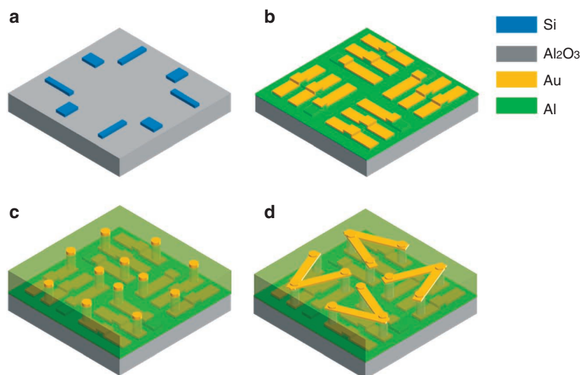
Figure 5 | Flowchart of the fabrication of the handedness switching metamaterials. (a) Patterning of silicon pads (blue) on top of the Al 2 O 3 substrate (gray) by photo-lithography and reactive ion etching. (b) Fabrication of gold pads on top of Al-coated silicon pads by a second photo-lithography followed by electron beam evaporation and lift-off process. (c) Coating of spin-on-glass and SU8 on the wafer, followed by patterning of holes in the SU8 by using photo-lithography and dry etching. Then, gold columns are created in the holes by electroplating. (d) Fabrication of gold bridges that connect the gold pillars by another photo-lithography process.
