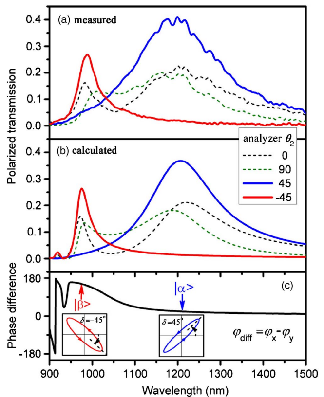
FIG. 3. (Color online) (a) Measured and (b) calculated transmission spectra with the polarization analyzer set at \theta_2 = 0^\circ, 45^\circ, 90^\circ , and -45^\circ , in the case of the polarizer of \theta_1 = 0^\circ . (c) Phase difference between the detected phases in x and y directions ( \varphi_{\text{diff}} = \varphi_x - \varphi_y ) as the function of the wavelength, where insets are the calculated polarization states of the transmitted light at two eigenfrequencies.
